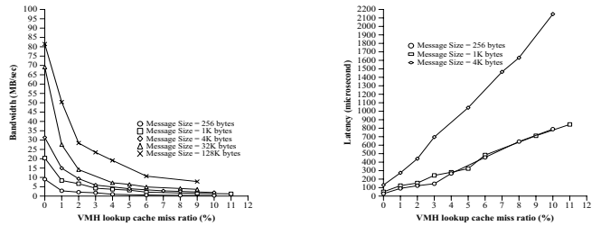
Fig. 4. The effect of VMH miss on ping-pong latency and bandwidth.
