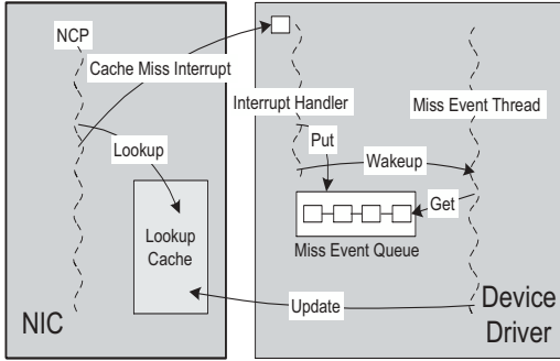
Fig. 1. Cache miss handling path.
