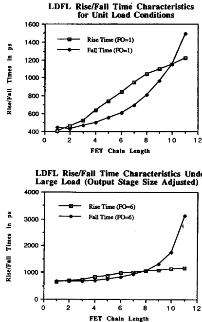
Figure 6. Rise/Fall Time Characteristics.
