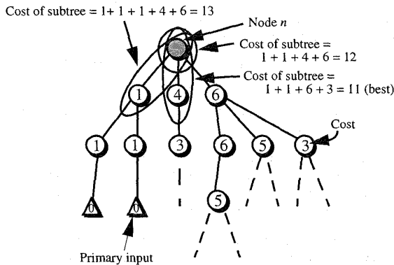
Figure 3. Computation of feasible subtree cost.
