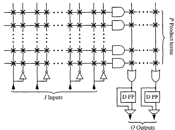
Figure 1. PLA-Style Logic Block.
