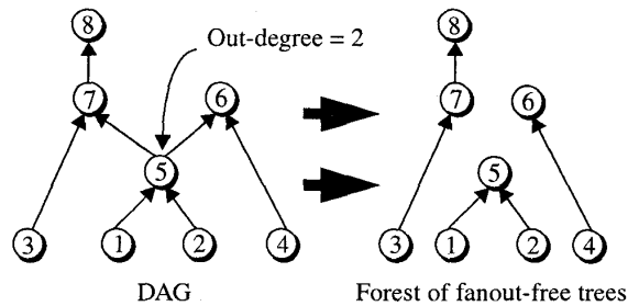
Figure 2. Partitioning a DAG into a forest of fanout-free trees. necessary to consider replication of logic at this juncture of the algorithm.
