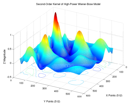
Figure 12: Second-Order Kernel of High-Power Wiener-Bose Model ( \alpha = 0.94 )
