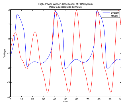
Figure 38: High-Power Wiener-Bose Model of FHN System ( 0.33\cos(0.33t) Stimulus)
