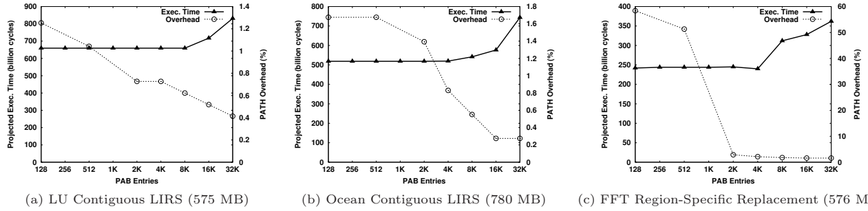
Figure 10: The effect of PAB size on the projected execution time and runtime overhead for page replacement algorithms.
