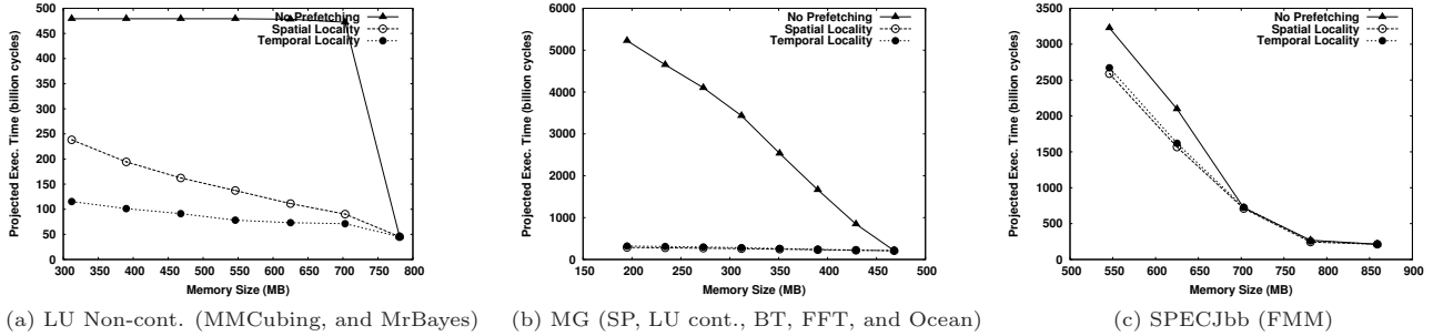
Figure 8: The effect of prefetching on the projected execution time. In parenthesis are applications which present similar behavior.
