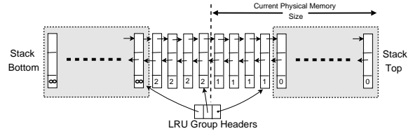
Figure 4: The optimized structure for LRU group headers.
