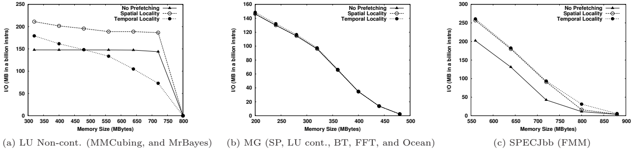
Figure 9: The effect of prefetching on the required I/O bandwidth. In parenthesis are applications which present similar behavior.
