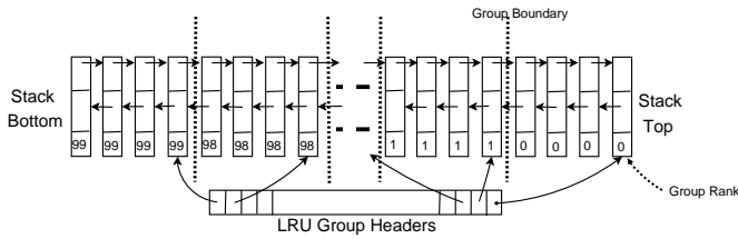
Figure 3: The LRU stack with group headers.
