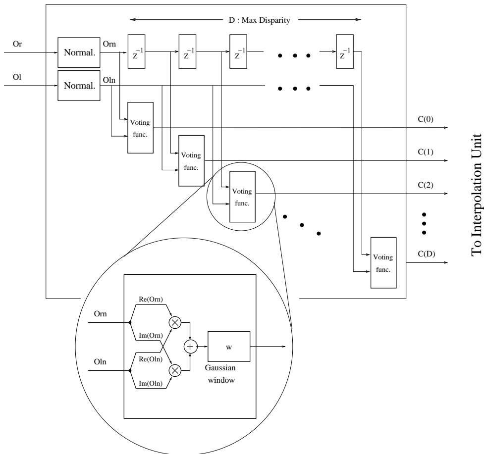
Figure 3.13: Extracting the normalizer blocks and sharing them across all voting functions reduces the complexity inside each voting function block.
