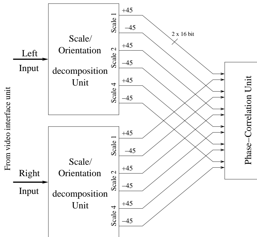
Figure 3.8: Communication between Scale/Orientation Unit and Correlation Unit
