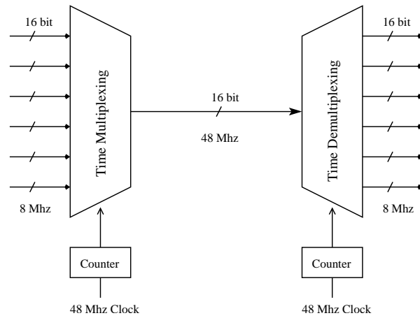
Figure 3.22: Time Multiplexing/Demultiplexing in chip-to-chip communication
