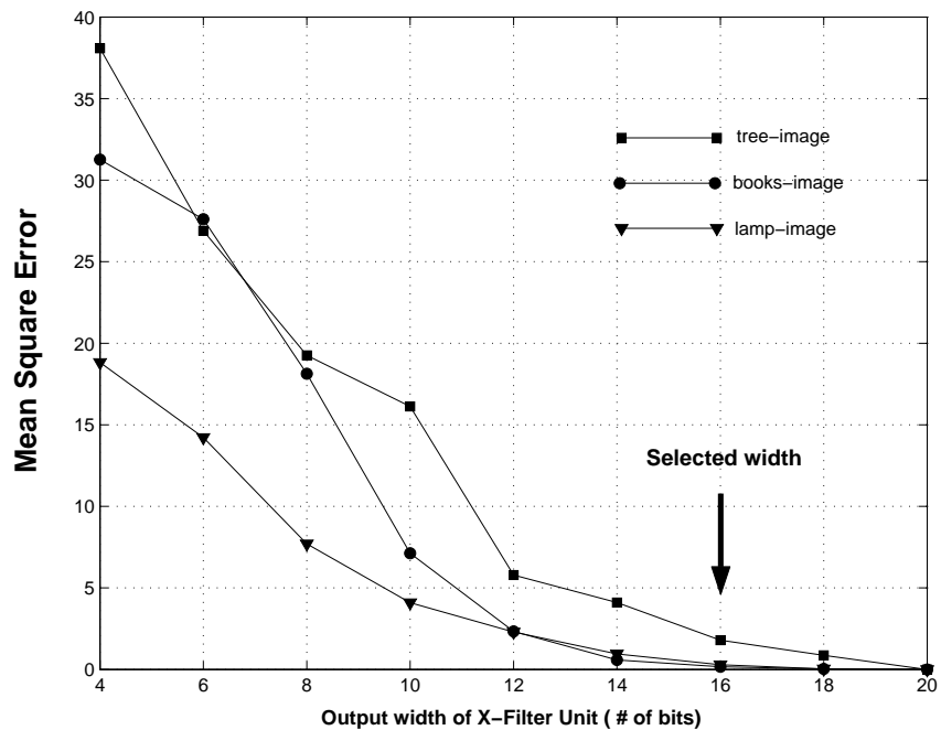
Figure 3.18: Fixed-point analysis for the X-filter block output width. Based on this analysis, we represent X-filter outputs with 16-bit signed values.
