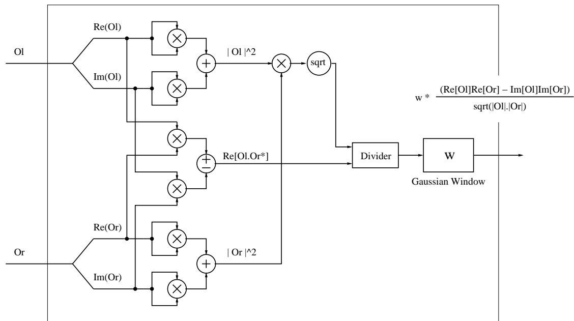
Figure 3.11: Revised voting function architecture: The Gaussian window is moved to the end of block
