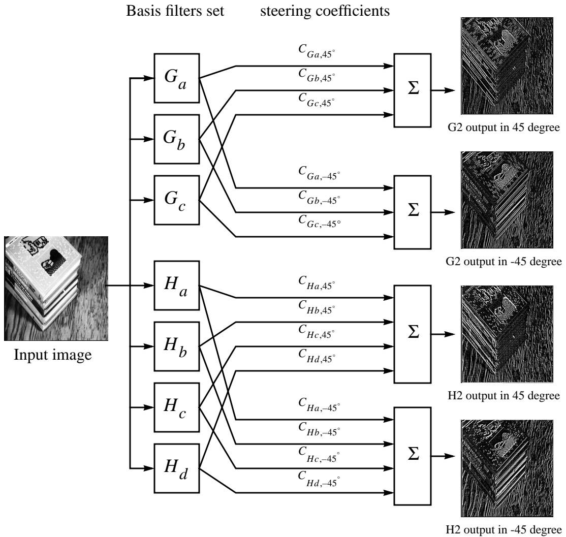
Figure 3.5: Architecture of the G2/H2 filter block. Any orientation of G2/H2 filters can be calculated by a linear combination of a set of seven basis filters.
