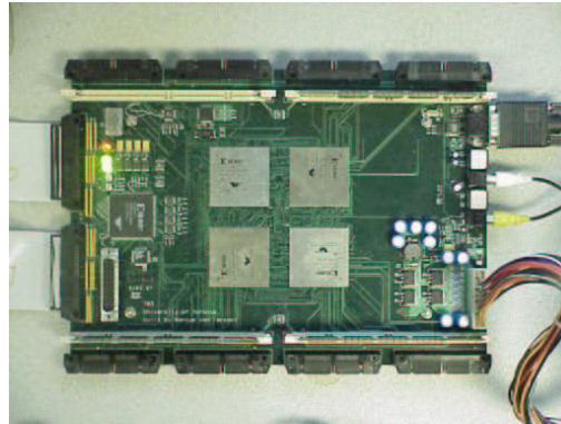
Figure 2.8: Transmogrieffier-3A board
