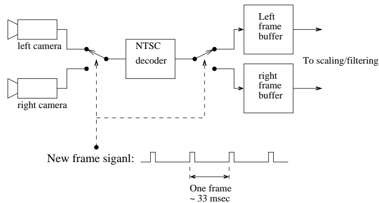
Figure 3.3: Using source selector to alternate between left and right cameras
