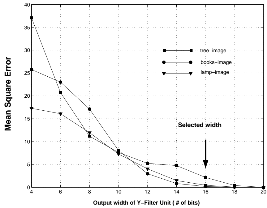
Figure 3.19: Fixed-point analysis for the Y-filter block output width. Based on this analysis, we represent Y-filter outputs with 16-bit signed values.
