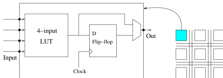
Figure 2.7: Simplified architecture of a logic block with one 4-input LUT and one flip flop. The flip flop at the output of LUT allows storage of the LUT output and hence implementing sequential circuits.
