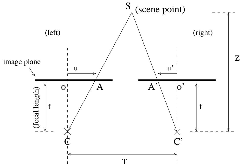
Figure 2.2: Calculating depth from disparity
