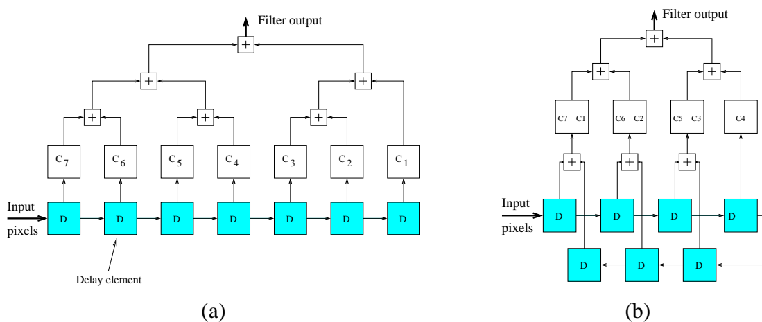
Figure 3.7: (a) Original architecture of the horizontal 7-tap FIR filter. (b) Revised architecture with symmetric coefficients. (For anti-symmetric coefficients the first level of adders can be replaced with subtractors.)
