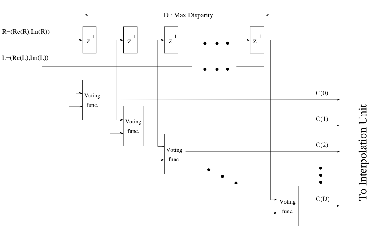
Figure 3.9: High level architecture of Phase-Correlation Unit for one pair of left and right images. In this architecture, all the voting function blocks are operating in parallel.
