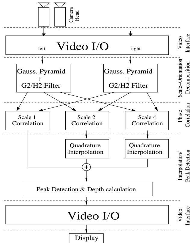
Figure 3.1: High Level Stereo System Architecture. Two video inputs are received from parallel cameras and are passed through multi-scale multi-resolution LWPC algorithm. The Video Output Interface sends the depth map results to display.
