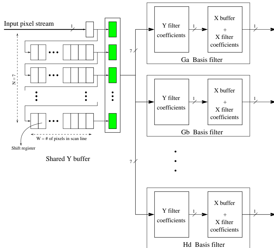
Figure 3.6: Sharing Y buffer for all seven Y filters of the basis filters. The Y buffers are by far larger than X buffers. So, sharing the Y buffer among all the basis filters saves more hardware as opposed to sharing X buffers.
