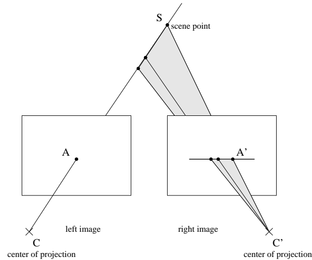
Figure 2.3: Epipolar Constraint
