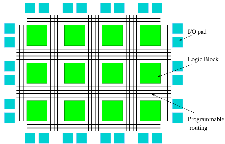
Figure 2.6: Architecture of a generic FPGA
