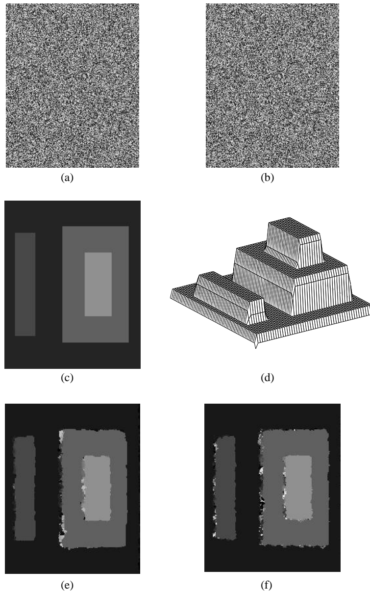
Figure 4.2: Overall system performance on a pair of random stereograms: (a), (b) Random-dot stereogram (c) Ground truth depth (d) 3D structure of ground truth (e) Depth from original software (f) Depth from hardware vision system
