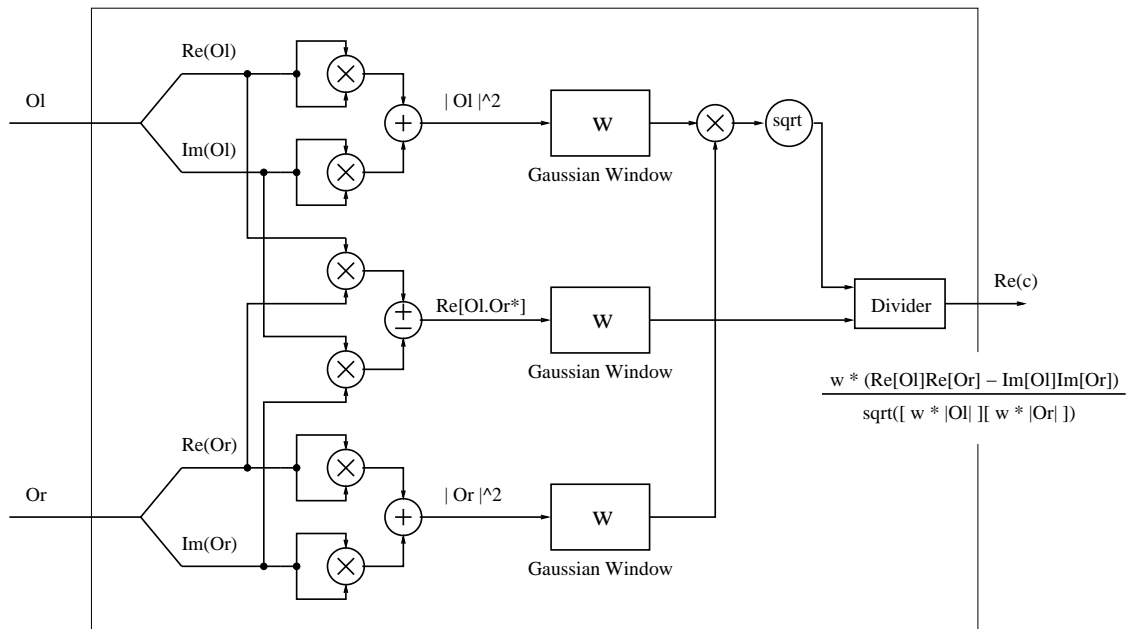
Figure 3.10: Realization of the real part of voting function in (3.4)
