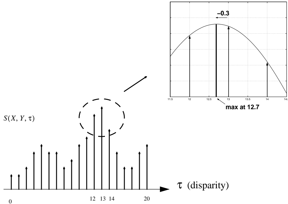
Figure 3.16: Sub-pixel accuracy in disparity is obtained by adding \Delta_{\tau} to the integer-valued \tau .
