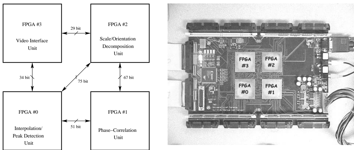
Figure 3.23: Data transfer between four FPGAs
