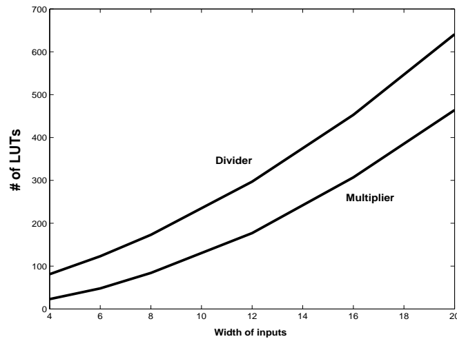
Figure 3.17: Divider and Multiplier Hardware Cost
