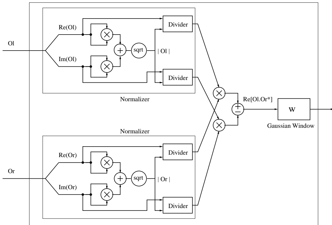
Figure 3.12: Re-arrangement of the architecture of Figure 3.11 with two normalizer blocks, one inner product and one Gaussian window unit.
