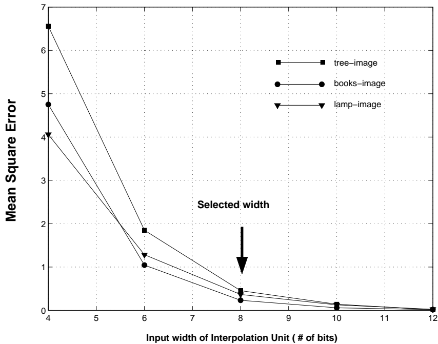
Figure 3.21: Fixed-point analysis for the input width of the Interpolation Unit (output of Phase-Correlation Unit). Based on this analysis, we represent Interpolation Unit inputs with 8-bit signed values.
