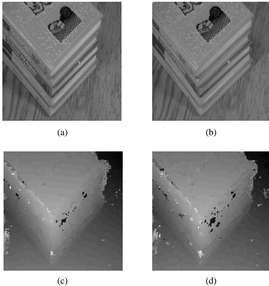
Figure 3.15: Effect of using L_1 -norm instead of L_2 -norm and changing the location of Gaussian window on the final depth map results of the ‘books’ stereo images. (a) Left image. (b) Right image. (c) Depth map by using L_2 -norm and original location for Gaussian window. (d) Depth map by using L_1 -norm and Gaussian window moved to the end of voting function block.
