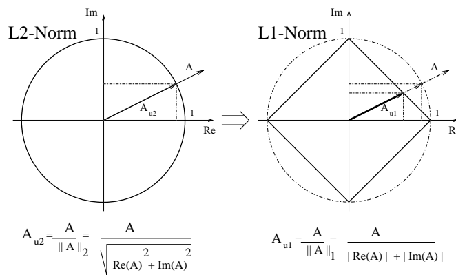
Figure 3.14: Effect of using L_1 -norm instead of L_2 -norm
