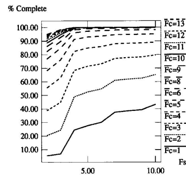
Fig. 10. Routability predictions versus F_s for circuit BNRE.
