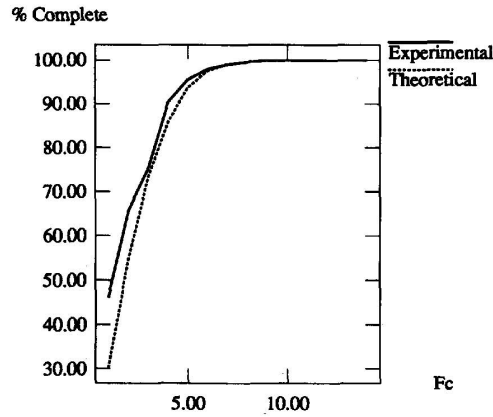
Fig. 11. Comparison of predictions and experiments for F_s = 6 .
