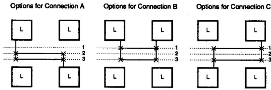
Fig. 3. An example routing problem.
