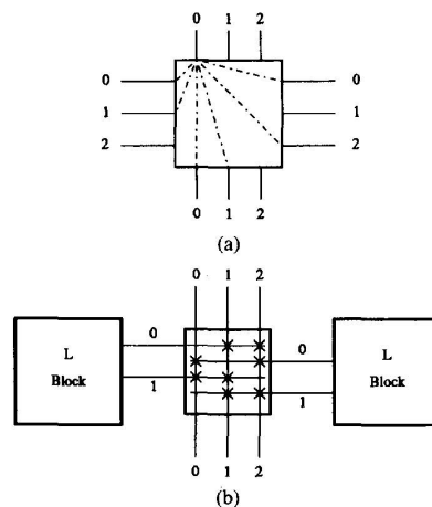
Fig. 2. Definition of (a) S and (b) C block flexibilities.
