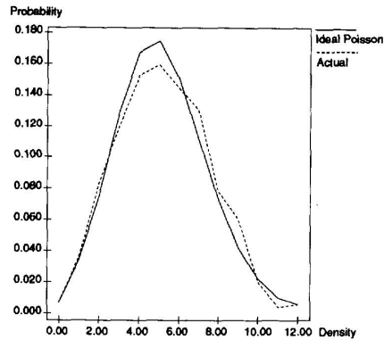
Fig. 4. Predicted versus actual channel densities.
