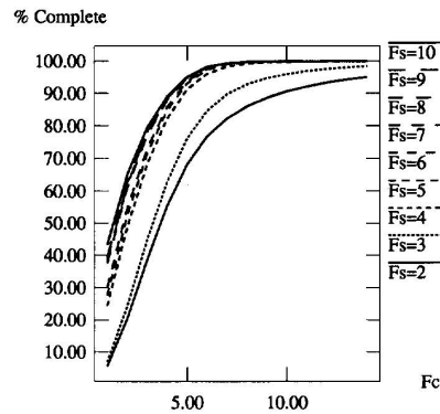
Fig. 9. Routability predictions versus F_c for circuit BNRE.
