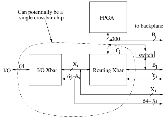
Figure 3.6 Use of Analog Switches to Reduce Pin Count on Crossbar Chip
