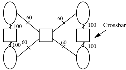
(c) Implementation of Circuit Using Crossbars
