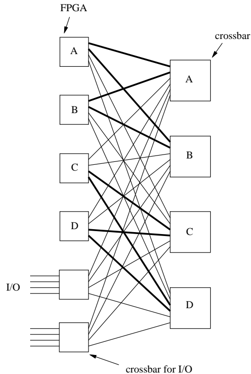
Figure 3.1 Partial Crossbar with Non-uniform Routing Density
