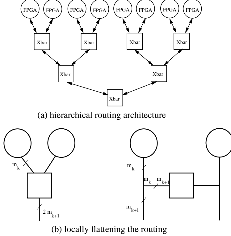
Figure 3.3 Flattening a Hierarchical Routing Architecture
