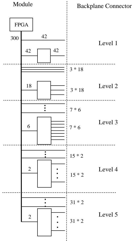
Figure 3.4 Routing Resource Distribution for 32
