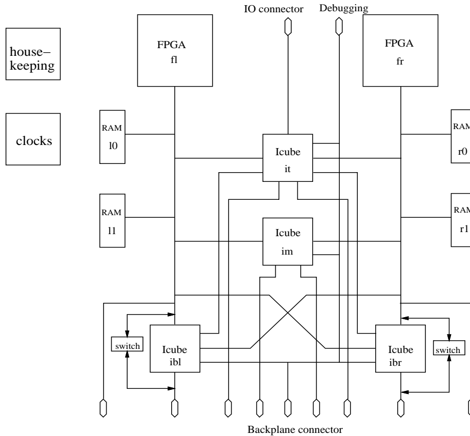
Figure 4.1 Organization of the TM-2 Printed Circuit Board
