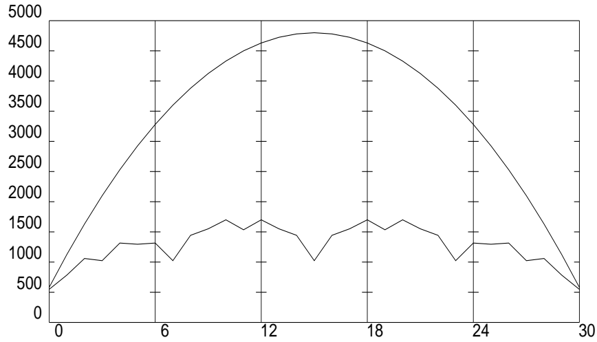
Figure 3.5 Wiring Density on Backplane
