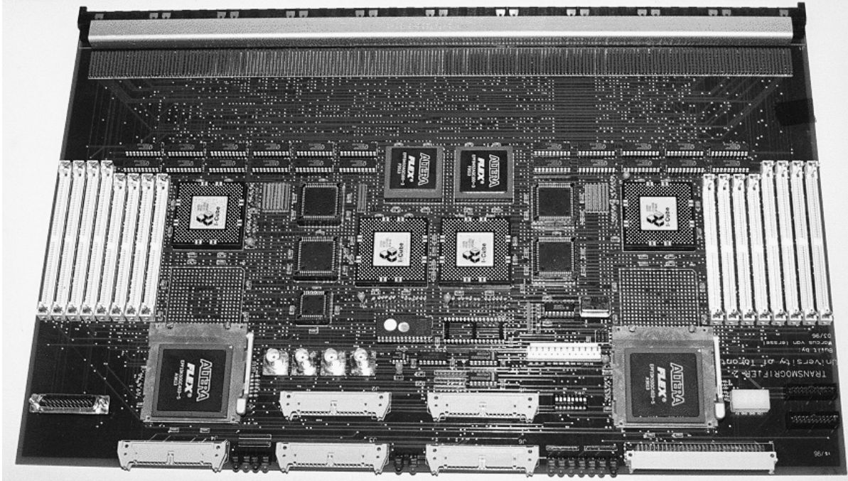
Figure 5.1 The TM-2 Printed Circuit Board
