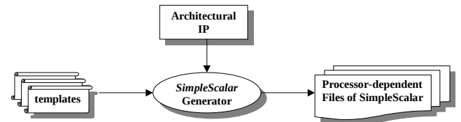
Figure 6: SimpleScalar Generator.
