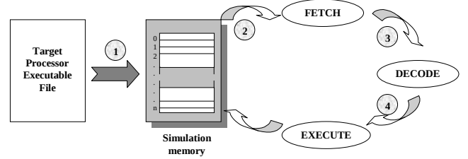
Figure 3: The Simple Simulation Process
