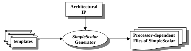
Figure 6: SimpleScalar Generator.
