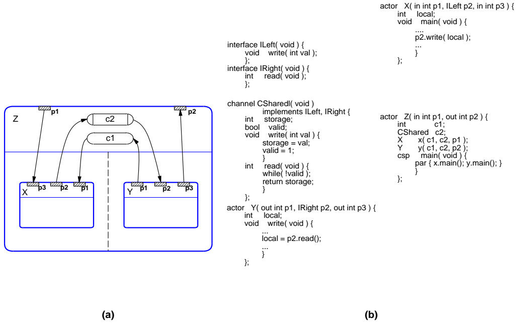
Figure 2: Basic structure of a SpecC+ program
