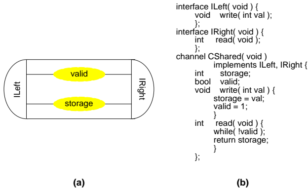
Figure 4: Shared memory channel
