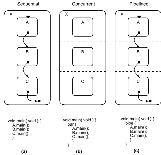
Figure 3: Behavioral hierarchy
