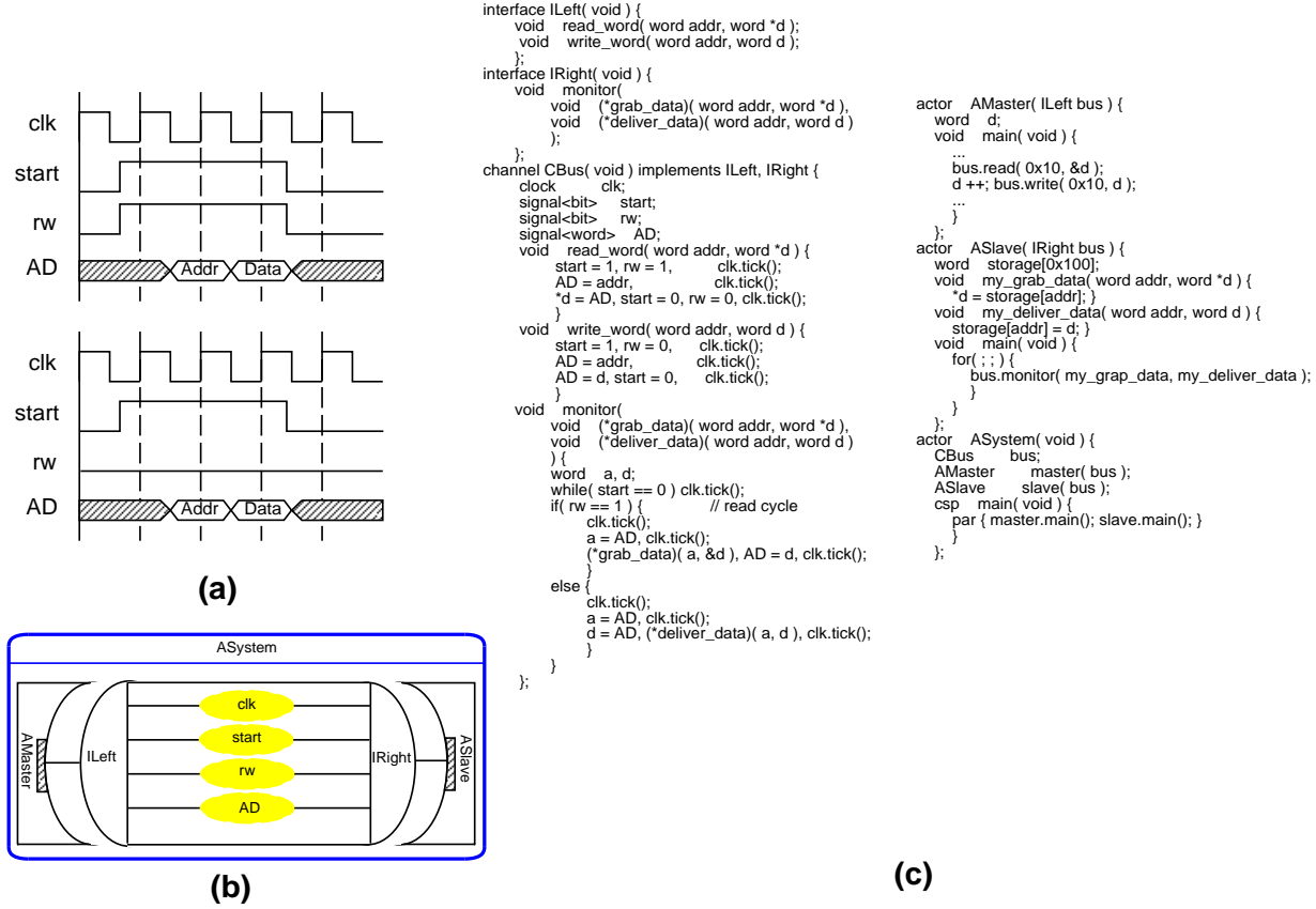
Figure 5: Synchronous bus channel
