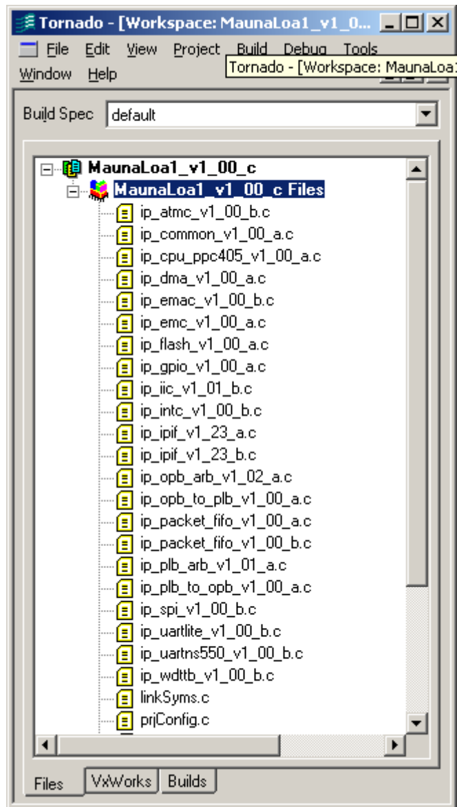
Figure 10-2: Tornado 2.x Project GUI - Files
