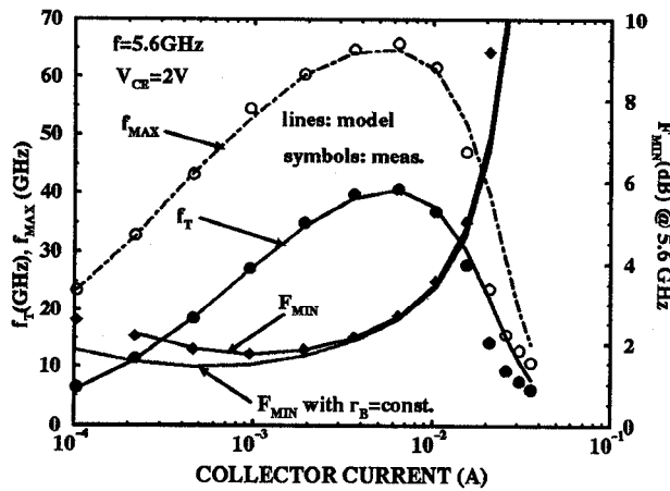
Fig.3: Measured (from Y parameters) vs. modeled f_T , f_{MAX} , and F_{MIN} for 0.5 \times 15 \mu\text{m}^2 SiGe HBT, showing impact of r_B modeling.
