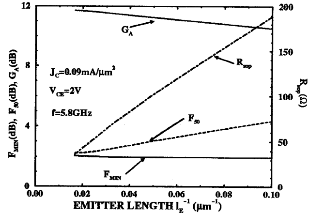
Fig.5: SGP-modeled noise parameters as functions of the emitter length, l_E , for the 0.5 \mu\text{m} emitter, NT25 double-poly Si bipolar process at 5.8GHz. F_{50} is the noise figure in a 50Ω system.
