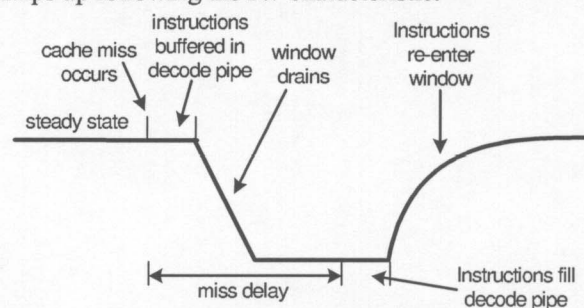
Figure 10: Instruction Cache Miss transient.
