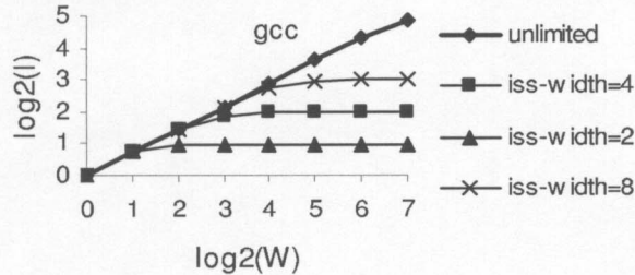
Figure 6: IW characteristic after limiting the issue width.
