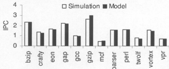
Figure 15: Comparison of performance predicted by our first-order model and from simulation.
