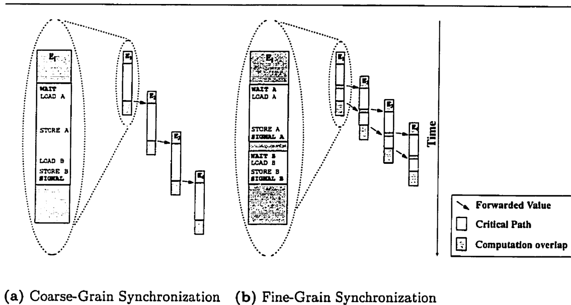
Figure 2.2: Examples of forwarding with coarse and fine grain synchronization.
