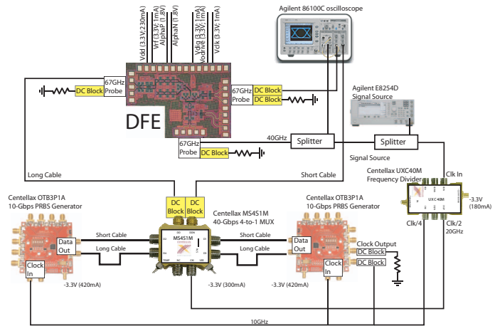
Fig. 10. Setup for large-signal 40-Gbps measurements
