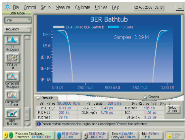
Fig. 14. Single-ended bathtub curve for single-ended output eye through 9-ft SMA cable at 39.5Gbps
