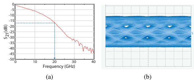
Fig. 11. 9-ft SMA cable (a) frequency response and (b) 40-Gbps input eye diagram
