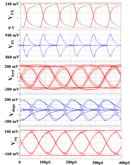
Fig. 2. Simulated eye diagrams at different nodes of the receiver at 15 Gb/s
