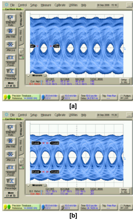
Fig. 4. Measured single ended 14 Gb/s output eye with a pattern length of 2^{31} - 1 ; [a] Linear path turned off (50 ps/div horizontal and 25 mv/div vertical); [b] Linear path activated (50 ps/div horizontal and 50 mv/div vertical).
