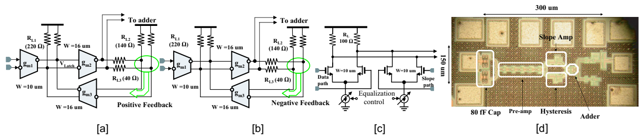
Fig. 3. Building blocks of the receiver front-end:(a) hysteresis (b) linear amplifier (c) Weighted summer. transconductors are simple NMOS diff pairs with minimum gate length (100-nm) drawn and device widths are as labeled (d) Die photo of AC receiver in 90-nm CMOS
