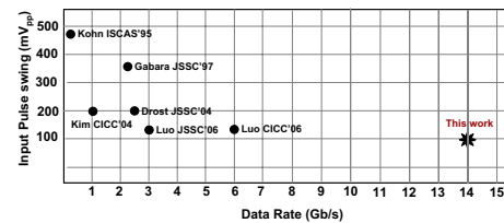
Fig. 6. Comparison of state-of-the art AC coupled receiver front-ends
