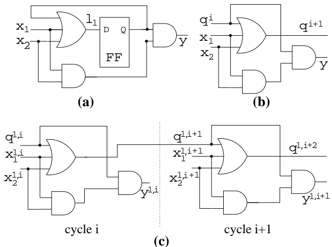
Figure 1: Example circuit
