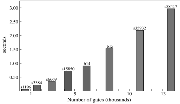
Figure 5: Run time vs. circuit size n
